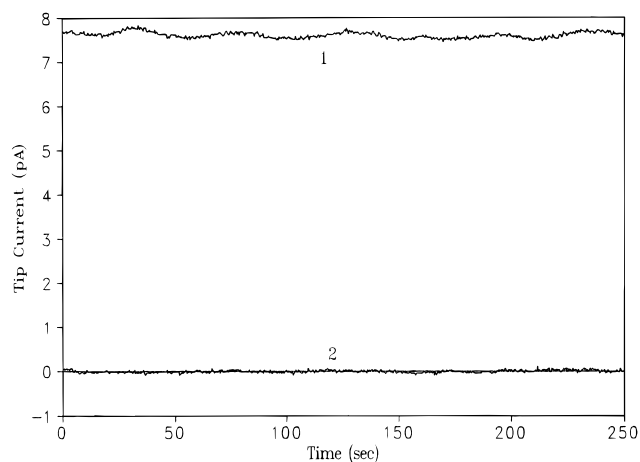
Figure 5. Tip current for a solution of 2 mM \text{CpFeCpTMA}^+ and 1.0 M \text{NaNO}_3 with a Pt–Ir tip at 0.6 V vs SCE and titanium dioxide substrate at (1) -0.7 and (2) 0.0 V vs SCE. d \approx 13 nm. Reprinted with permission from ref. 8. Copyright 1996 American Chemical Society.
